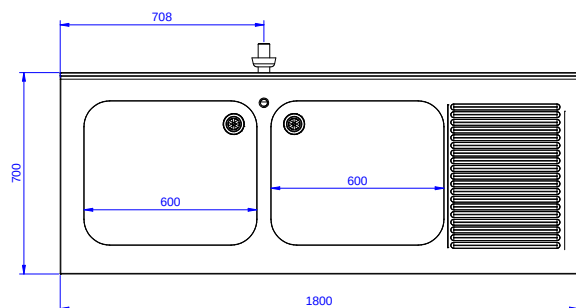
Shora
